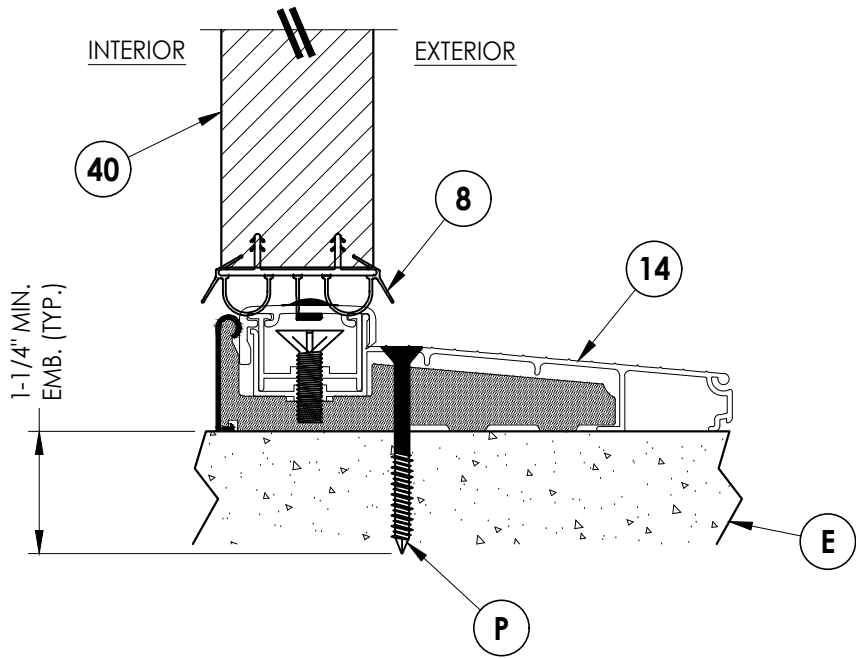
1 VERTICAL CROSS SECTION 9 Inswing Threshold
