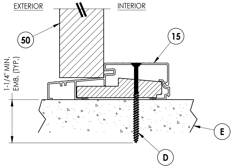
4 VERTICAL CROSS SECTION 9 Outswing Threshold
