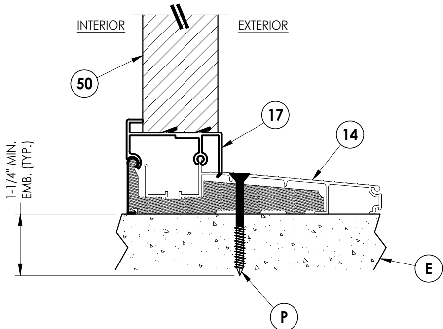
3 VERTICAL CROSS SECTION 9 Inswing Threshold
